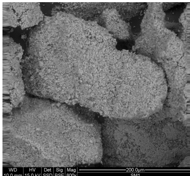
Phot. 12. The limestone from the zone of Mesozoic-Neogene contact in Bełchatów deposit (0.125–0.250 mm fraction). The grain surface after the calcinations process, lack of cracks (SEM/EDX)
